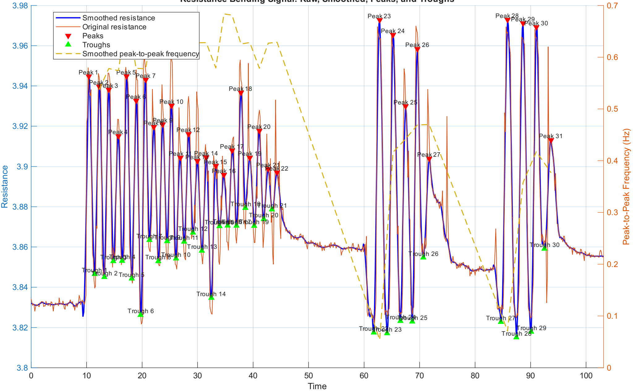
Resistance Bending Signal: Raw, Smoothed, Peaks, and Troughs
